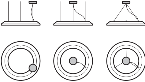
4246-XX Canopy on mounting point (STD) 4246-XX RCC Canopy centered with luminaire 4246-XX RCA Canopy centered with luminaire
